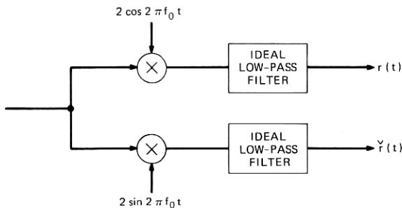
Fig. 5—Receiver “front end.”
