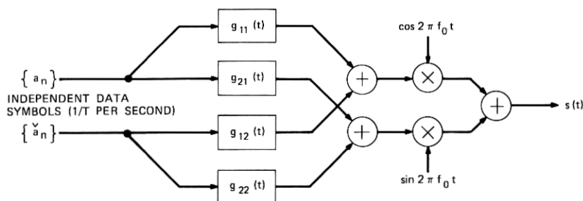
Fig. 3—General QAM transmitter structure.
